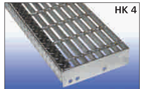
BOLTED fixing, holed end plates, floor plate nosing
